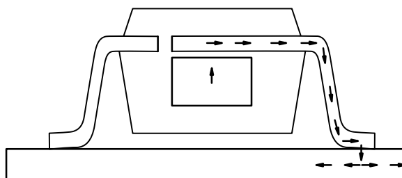
Figure 4. Thermal Path
